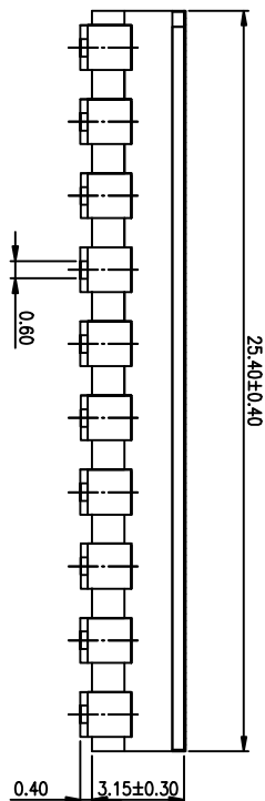
[Schematic]
